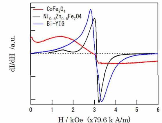
Fig. The ESR spectra of \text{CoFe}_2\text{O}_4 , (\text{Ni}_{0.5}\text{Zn}_{0.5})\text{Fe}_2\text{O}_4 and Bi-YIG aerogel composite specimens at 9.4 GHz.
