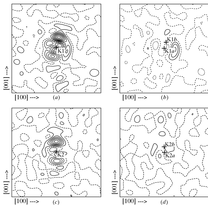
Figure 1 \Delta\rho maps in the (010) plane through the K1 and K2 sites for model I with unsplit sites (a, c) and model II with split sites (b, d). Contour intervals are 0.2 e Å −3 [ \sigma(\Delta\rho) = 0.08 \text{ e } \text{\AA}^{-3} ]. The positive and negative contours are shown as solid and short dashed lines, respectively. Map borders are 4 × 4 Å.
