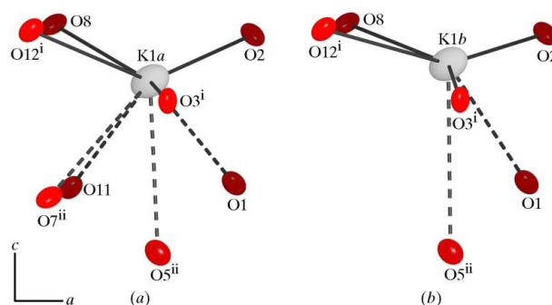
Figure 2 (a) The K1a and (b) the K1b coordination polyhedra, with displacement ellipsoids drawn at the 80% probability level. Symmetry codes are as given in Table 1.
