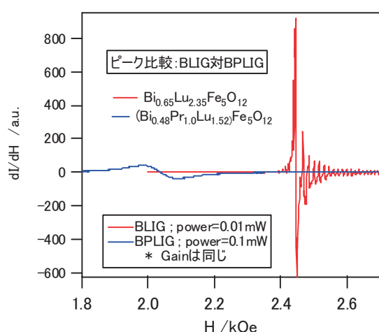
Fig.4. FMR spectra of (\text{BiLu})_3\text{Fe}_5\text{O}_{12} and (\text{BiPrLu})_3\text{Fe}_5\text{O}_{12} .
