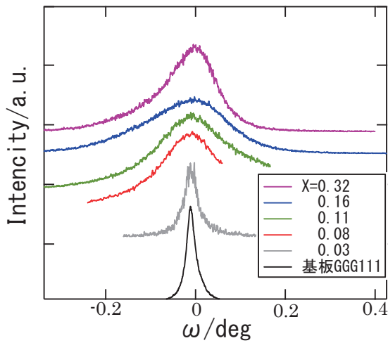
Fig.6. Rocking curve of 888 diffraction peaks of \text{Bi}_y\text{Pr}_x\text{Lu}_{3-x-y}\text{Fe}_5\text{O}_{12} films
